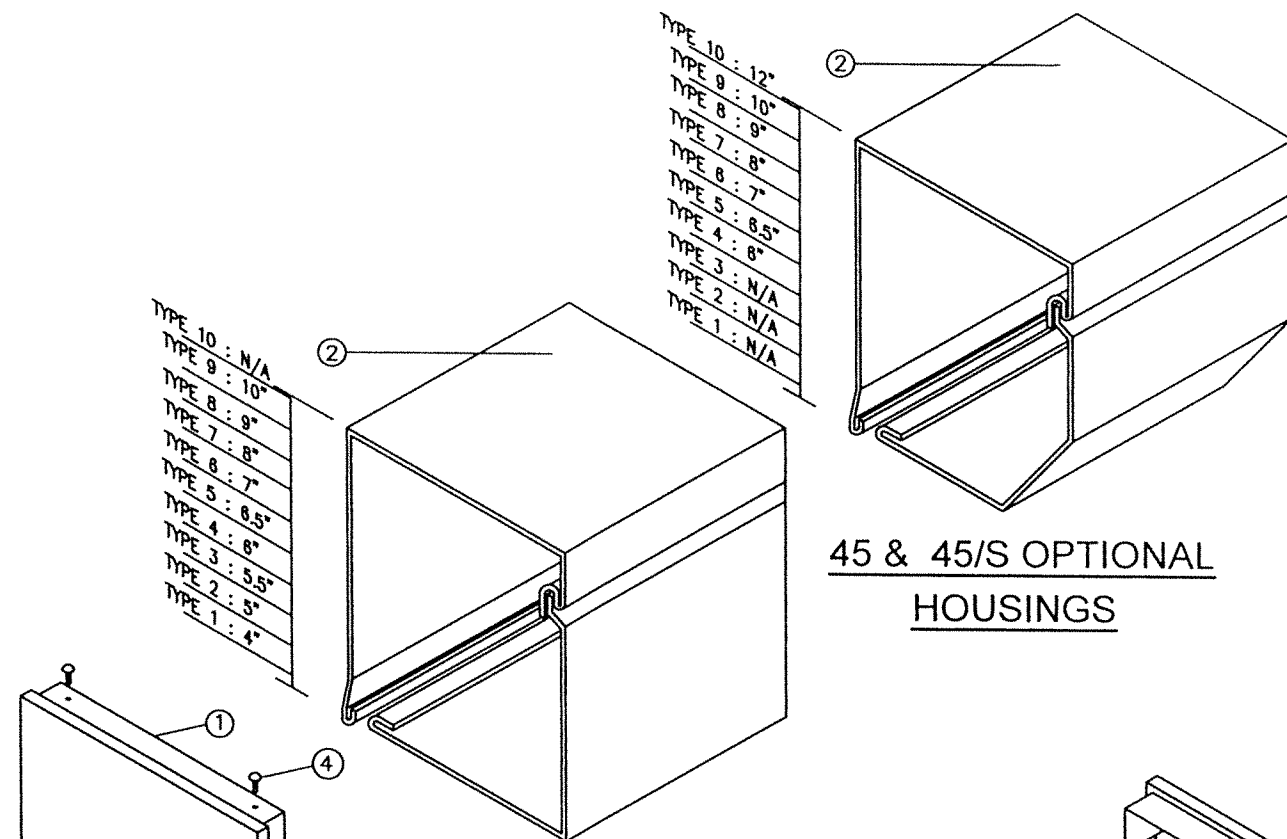
90 HOUSING
