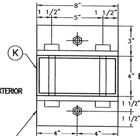
SECTION X1-X1 W/ (J)* (END & INTERIOR MULLION) (W/ ORIENTATION # 1) (6"x4")
