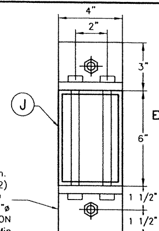
SECTION X1-X1 W/ (J)* (END & INTERIOR MULLION) (W/ ORIENTATION # 1) (6"x4")
